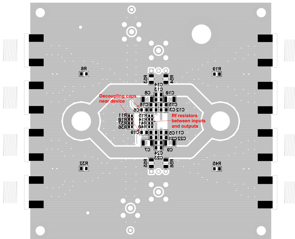
Figure 103. THS4532 EVM Bottom Layer 4
