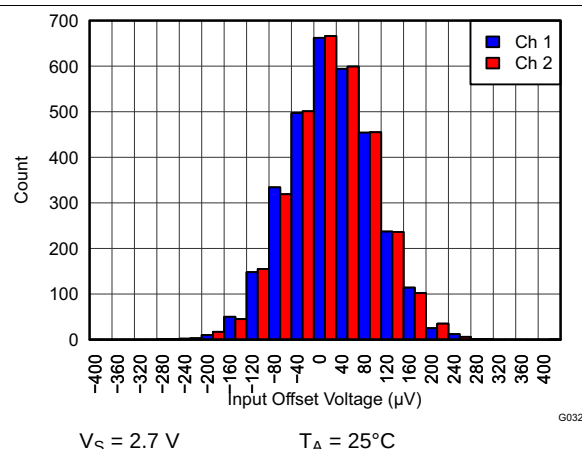
Figure 32. THS4532IPW Input Offset Voltage Histogram
