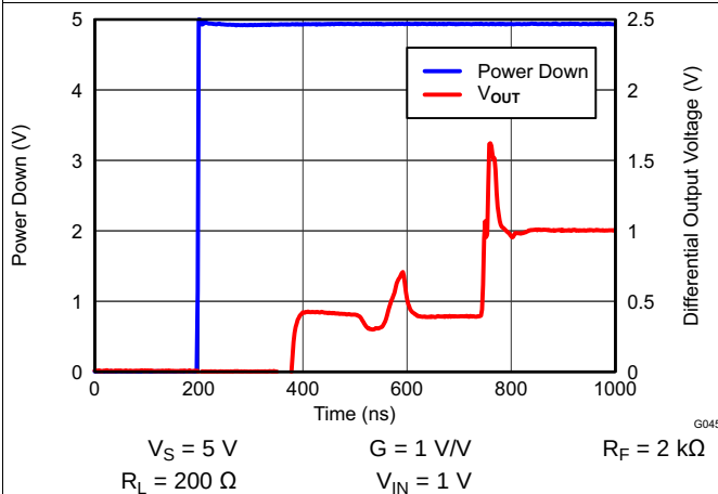
Figure 55. Turn-On Time
