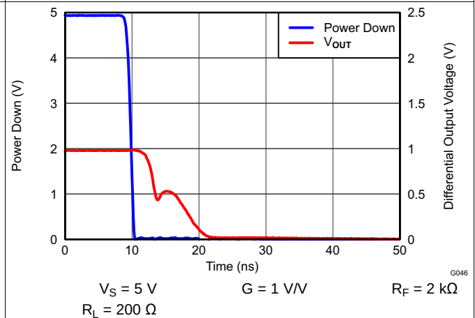
Figure 56. Turn-Off Time
