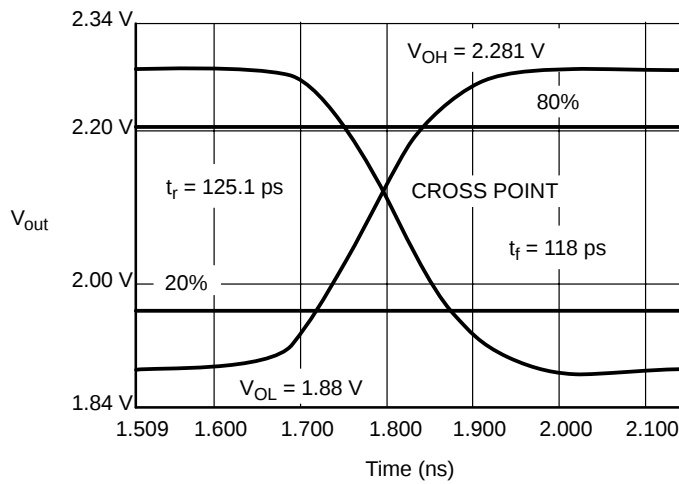
Figure 19. OBUF09 Reduced Swing Output Waveform (EP40/140)
