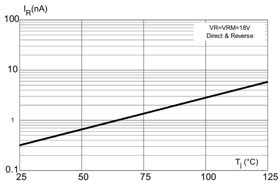
Figure 3. Leakage current versus junction temperature (typical values)
