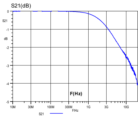
Figure 7. S21 attenuation
