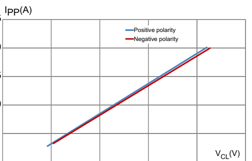
Figure 8. TLP measurements
