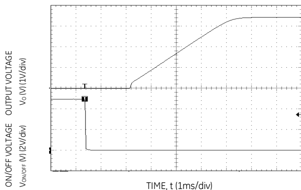
Figure 29. Typical Start-up Using On/Off Voltage ( I_o = I_{o,max} ).
