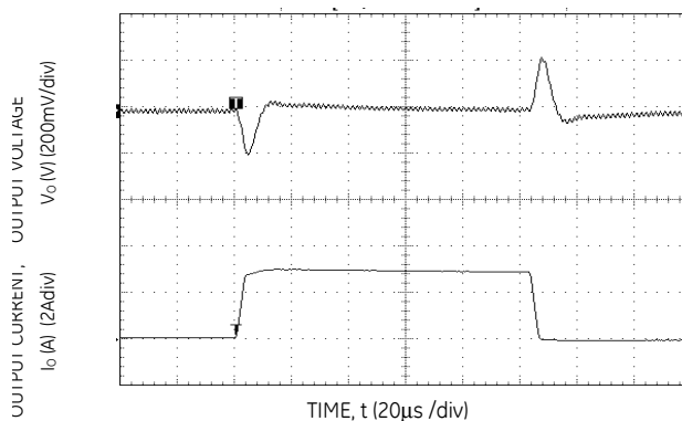
Figure 28. Transient Response to Dynamic Load Change from 0% to 50% to 0% with V_{IN}=5V .
