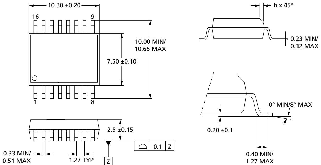
Figure 30: S016W 300 mils Body Width
