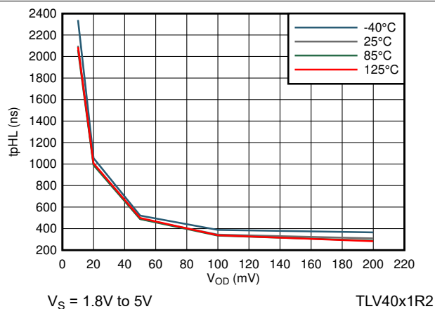
V_S = 1.8\text{ V to } 5\text{ V} TLV40x1R2 Figure 7-29. Propagation Delay High-Low vs Input Overdrive
