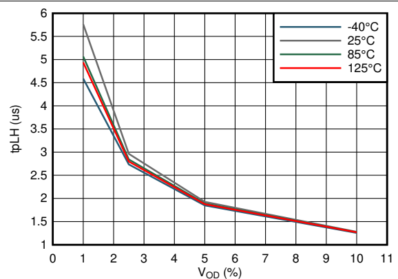
V_S = 1.8\text{ V to } 5\text{ V} TLV4021Sx5 Figure 7-30. Propagation Delay Low-High vs Input Overdrive
