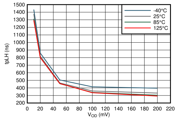
V_S = 1.8\text{ V to } 5\text{ V} TLV40x1R2 Figure 7-28. Propagation Delay Low-High vs Input Overdrive
