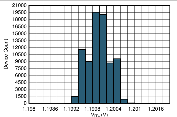
Figure 7-2. Positive Threshold Histogram
