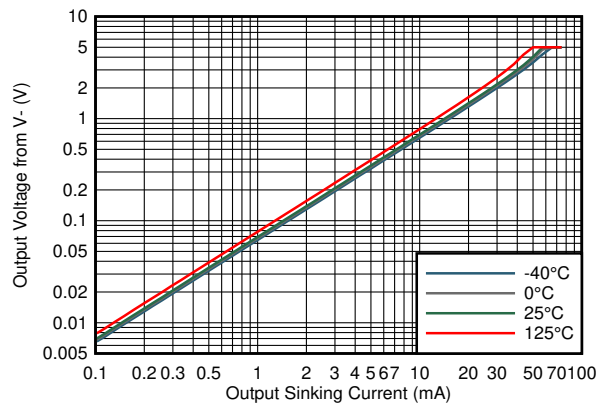
V_S = 5\text{ V} Figure 7-25. Output Voltage vs Output Sinking Current
