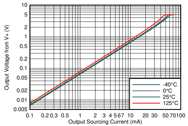
V_S = 5\text{ V} Figure 7-26. Output Voltage vs Output Sourcing Current
