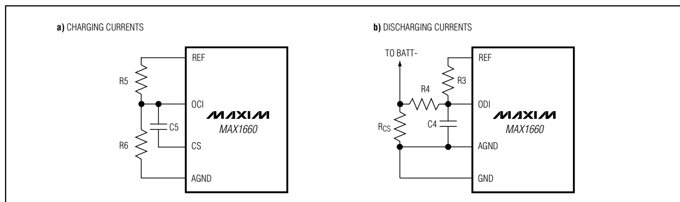
Figure 10. Overcurrent-Detection Networks
