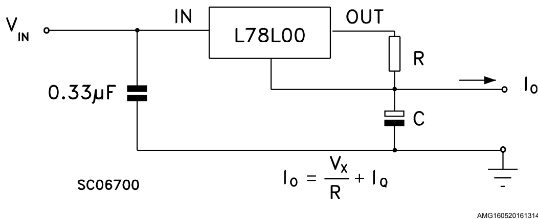
Figure 15. Current regulator
