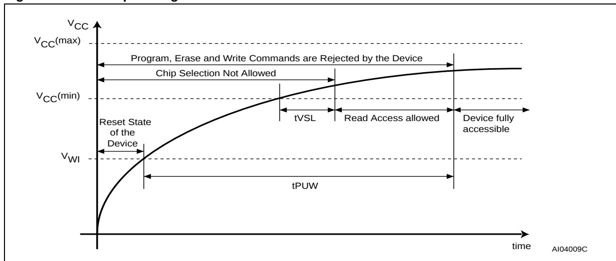
Figure 19. Power-up Timing
