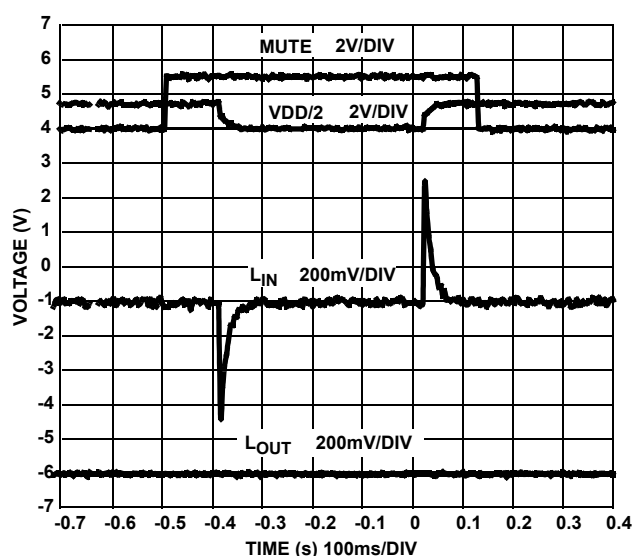
FIGURE 27. 32Ω AC COUPLED CLICK/POP REDUCTION
