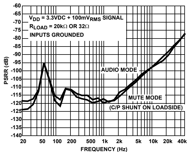
FIGURE 24. PSRR vs FREQUENCY
