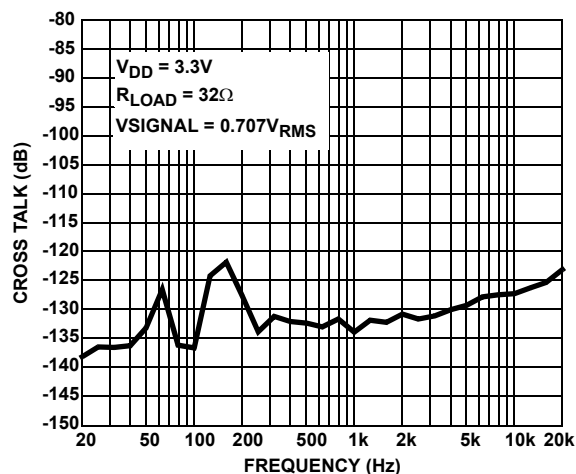
FIGURE 14. CHANNEL-TO-CHANNEL CROSSTALK
