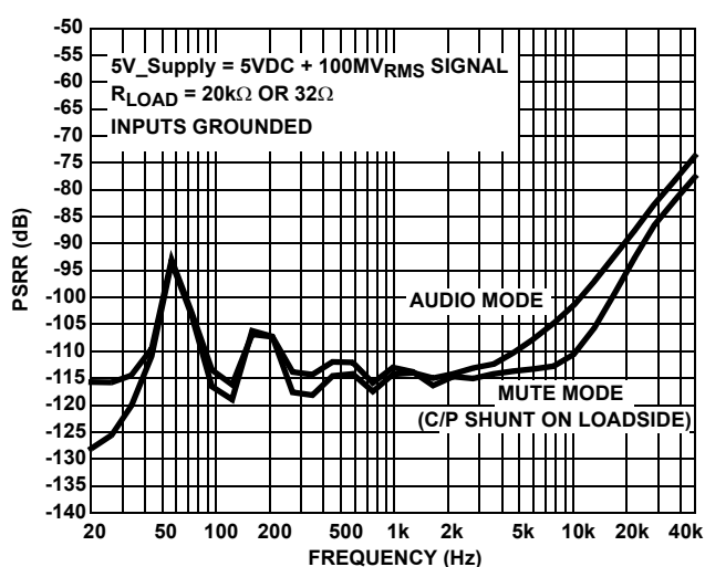
FIGURE 25. PSRR vs FREQUENCY
