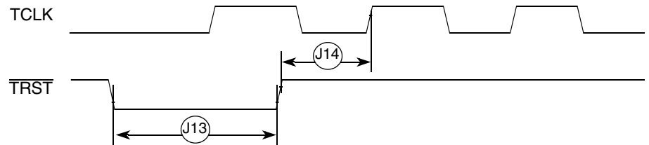
Figure 40. \overline{\text{TRST}} timing
