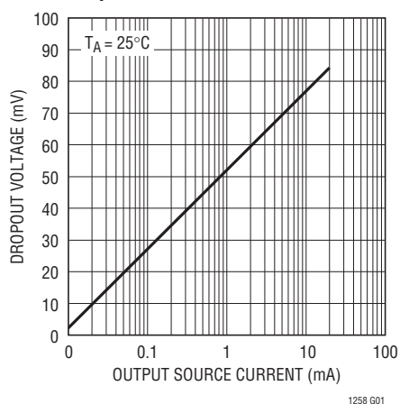
LTC1258-2.5* Dropout Voltage vs Output Source Current
