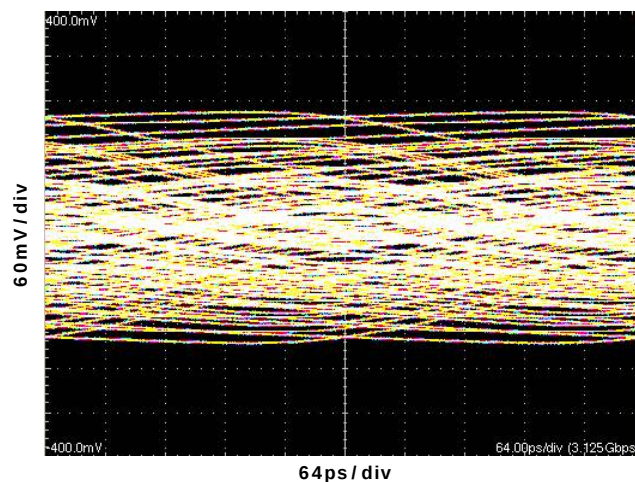
FIGURE 9. RECEIVED SIGNAL AFTER 25m OF 26AWG TWIN-AXIAL CABLE, 3.125Gb/s
