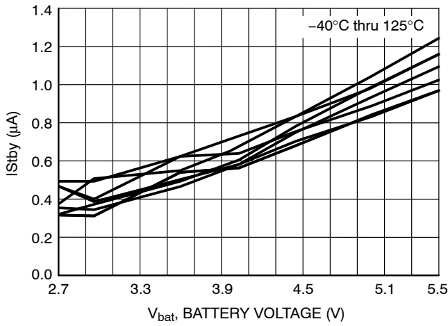
Figure 20. Standby Current
