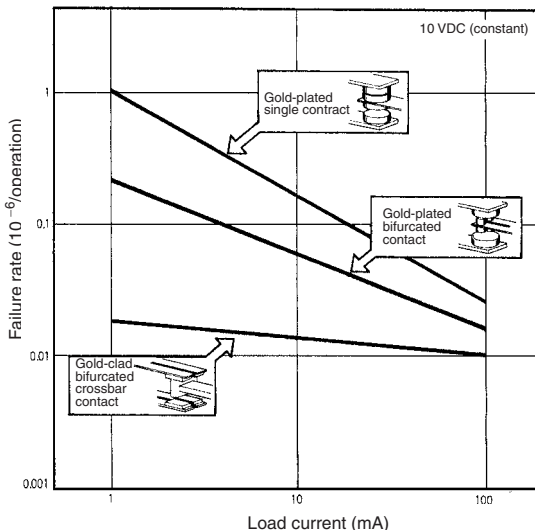
Failure Rate vs. Load Current
