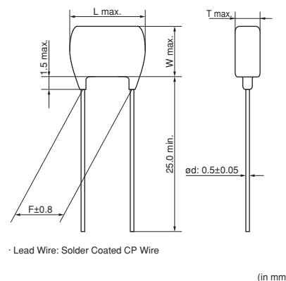
Dimensions code: 0 Lead style code: A2
