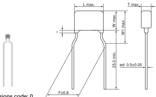
Dimensions code: 0 Lead style code: K1
