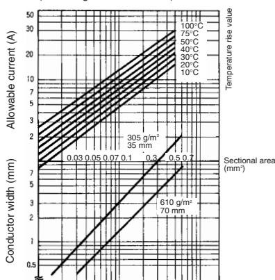
Conductor Width and Carry Current (according to IEC Pub326-3)
