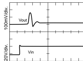
16 to 40 V MFL2805S Step Line Response
