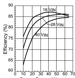
MFL2828S Efficiency
