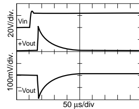
16 to 40 V MFL2815D Step Line Response
