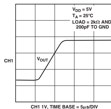
Figure 16. Half-Scale Settling (1/4 to 3/4 Scale Code Charge)
