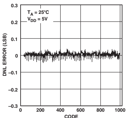
Figure 6. AD5311 Typical DNL Plot
