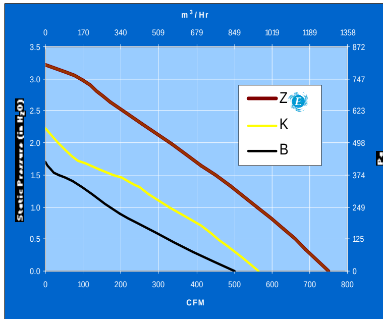
PERFORMANCE GRAPH
