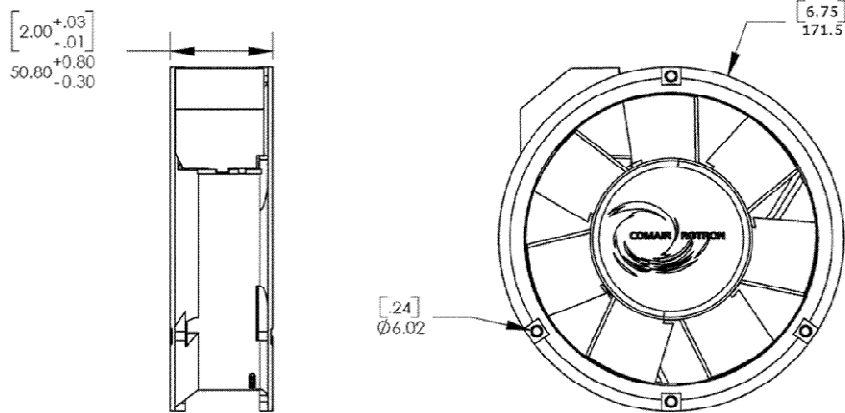
MECHANICAL DRAWING
