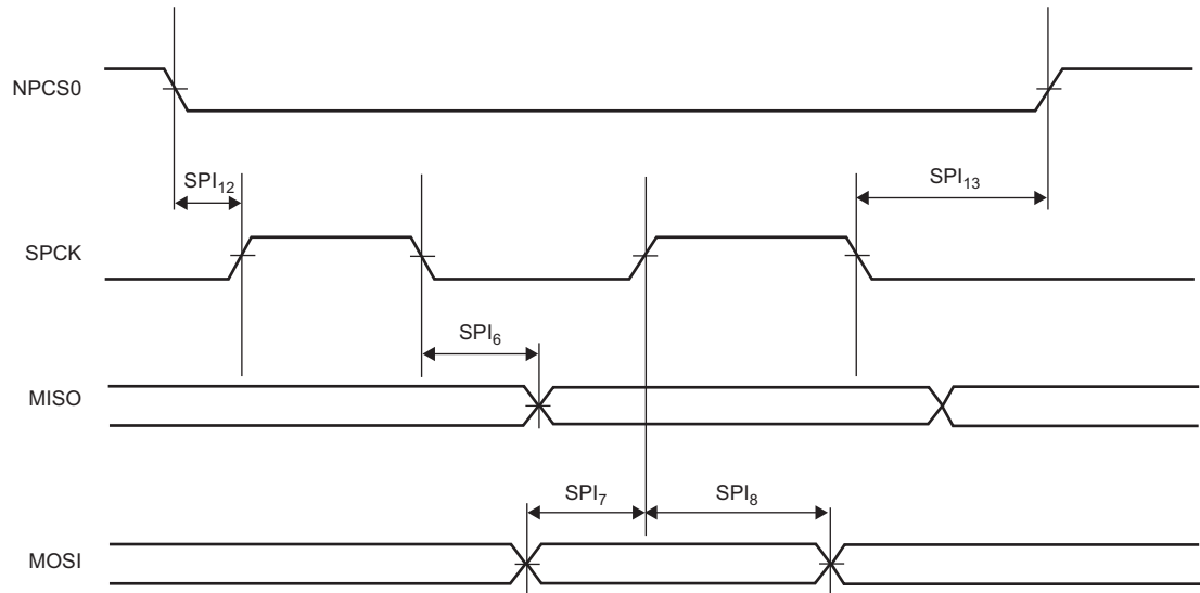
Figure 66-14: FLEXCOM in SPI Slave Modes 0 and 3
