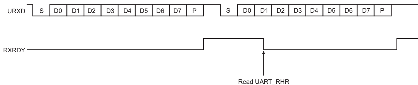
Figure 48-5: Receiver Ready
