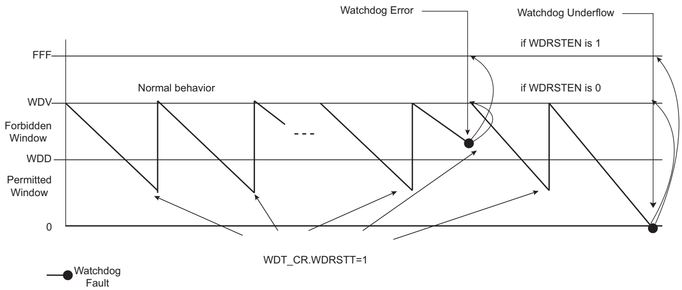
Figure 22-2: Watchdog Behavior
