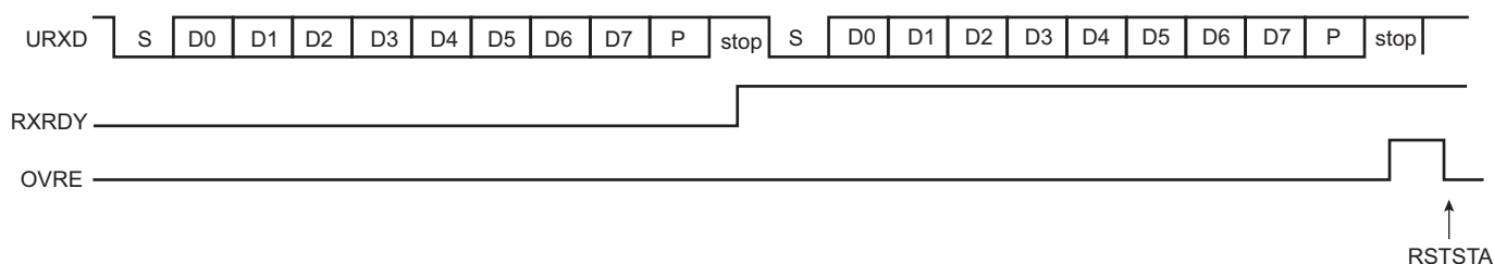
Figure 48-6: Receiver Overrun
