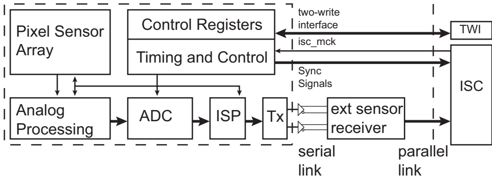
Figure 52-8: Serial CMOS Sensor with External Parallel Bridge
