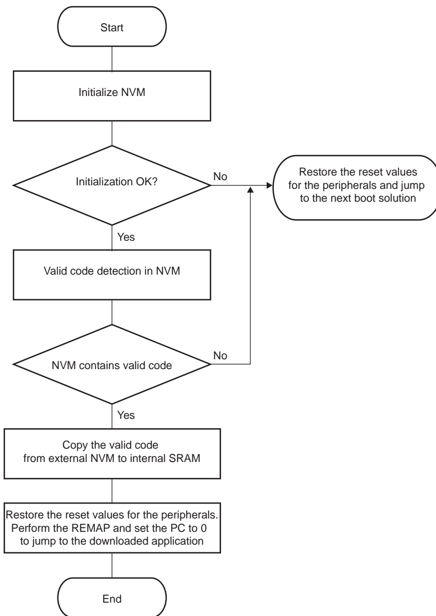
Figure 16-5: NVM Boot Diagram
