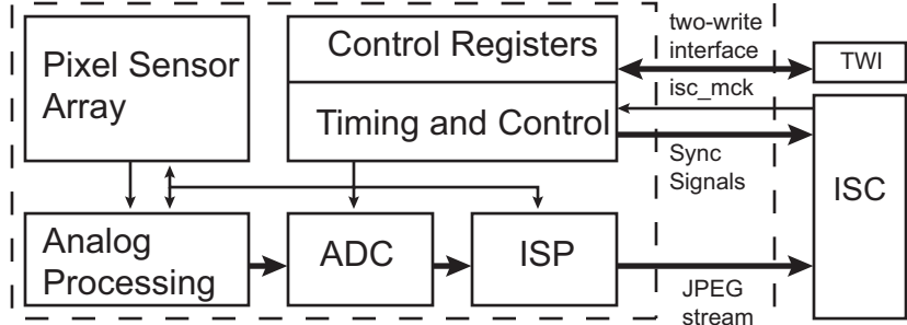
Figure 52-7: Sensor with JPEG Output
