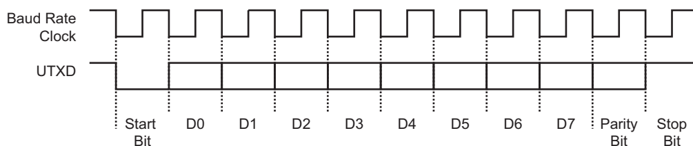
Figure 48-10: Character Transmission
