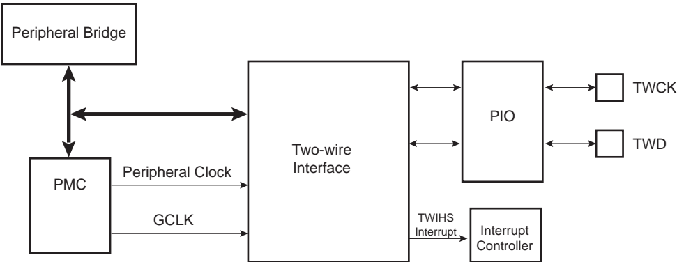
Figure 46-1: Block Diagram
