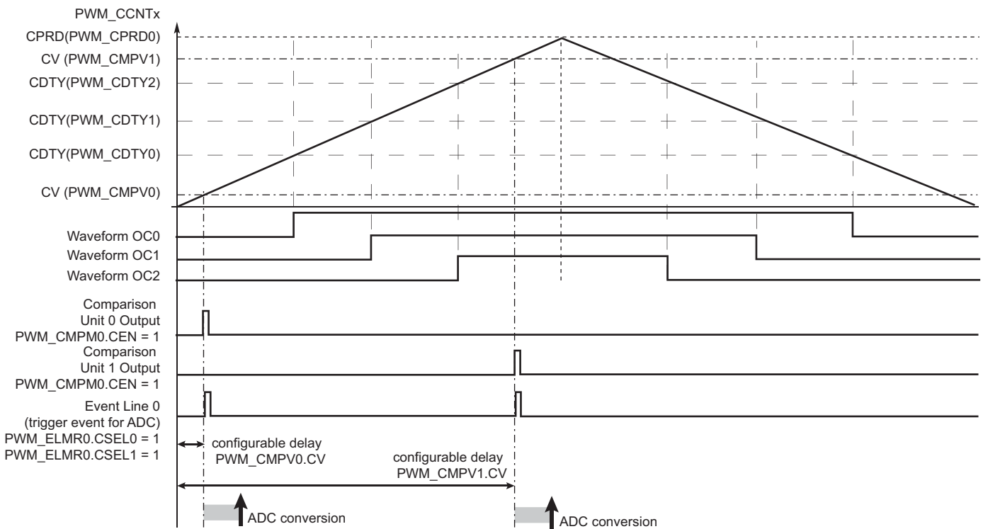
Figure 56-26: Event Line Generation Waveform (Example)
