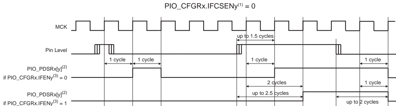
Figure 34-4: Input Glitch Filter Timing
