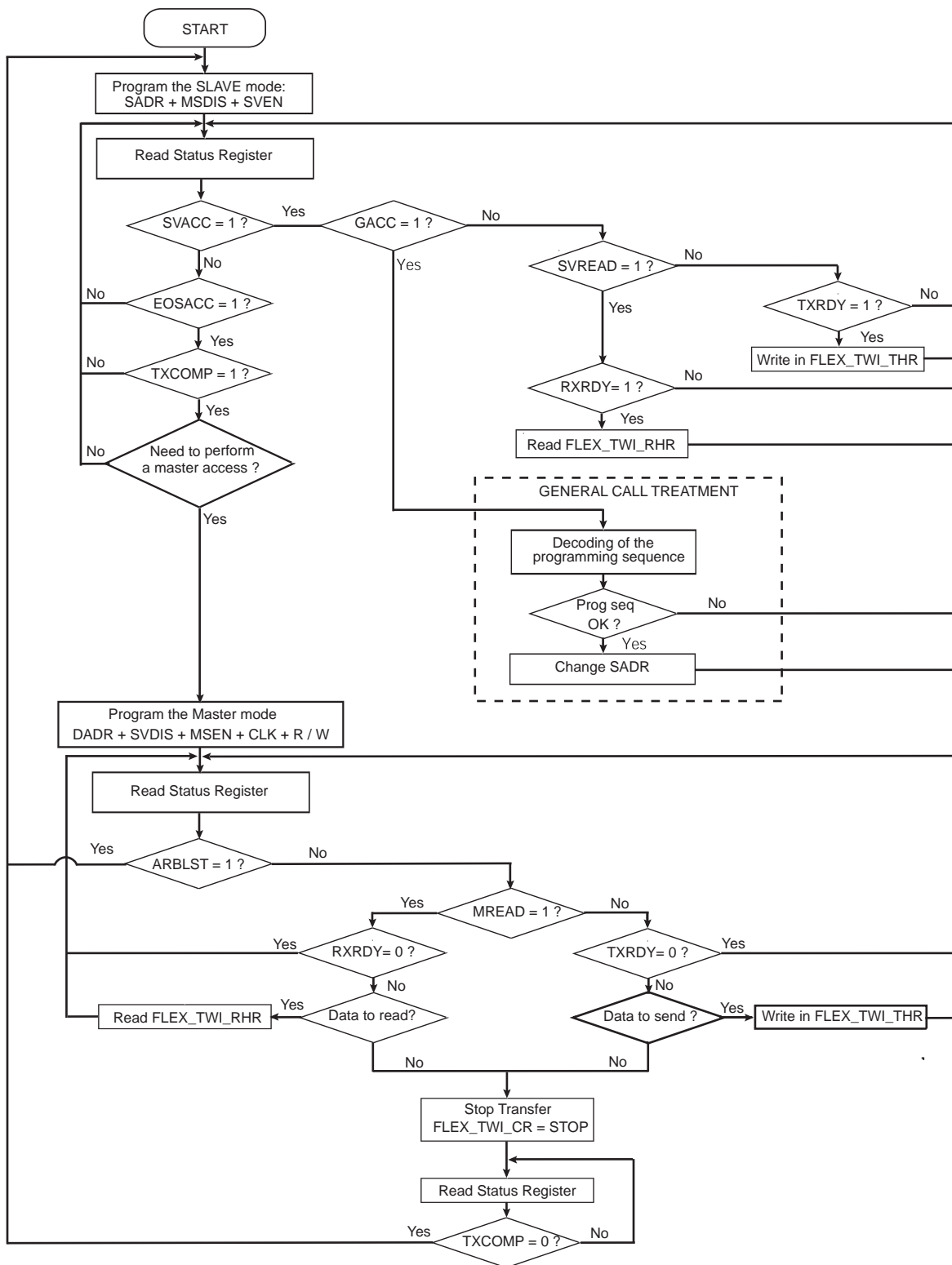
Figure 47-112: Multi-Master Mode
