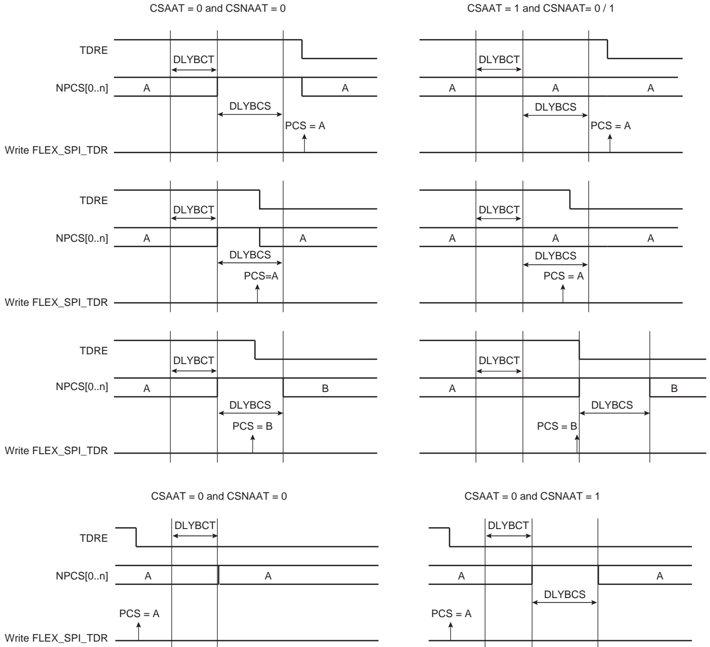
Figure 47-73: Peripheral Deselection
