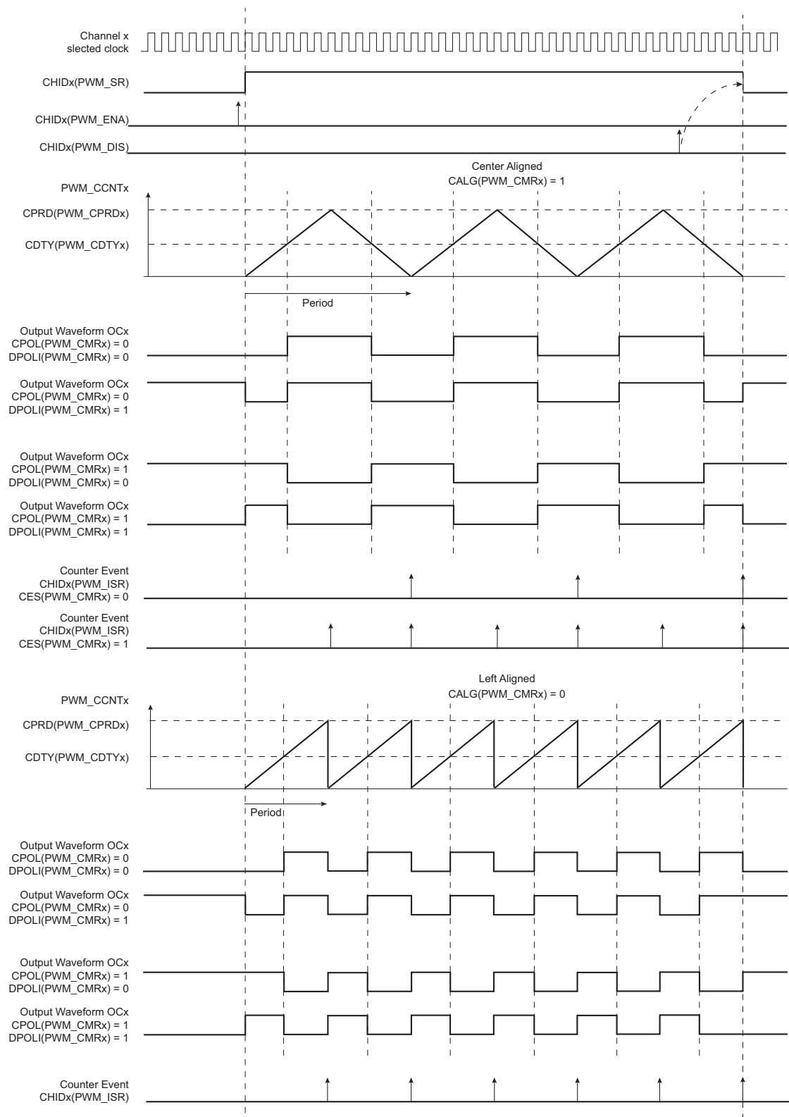
Figure 56-5: Waveform Properties
