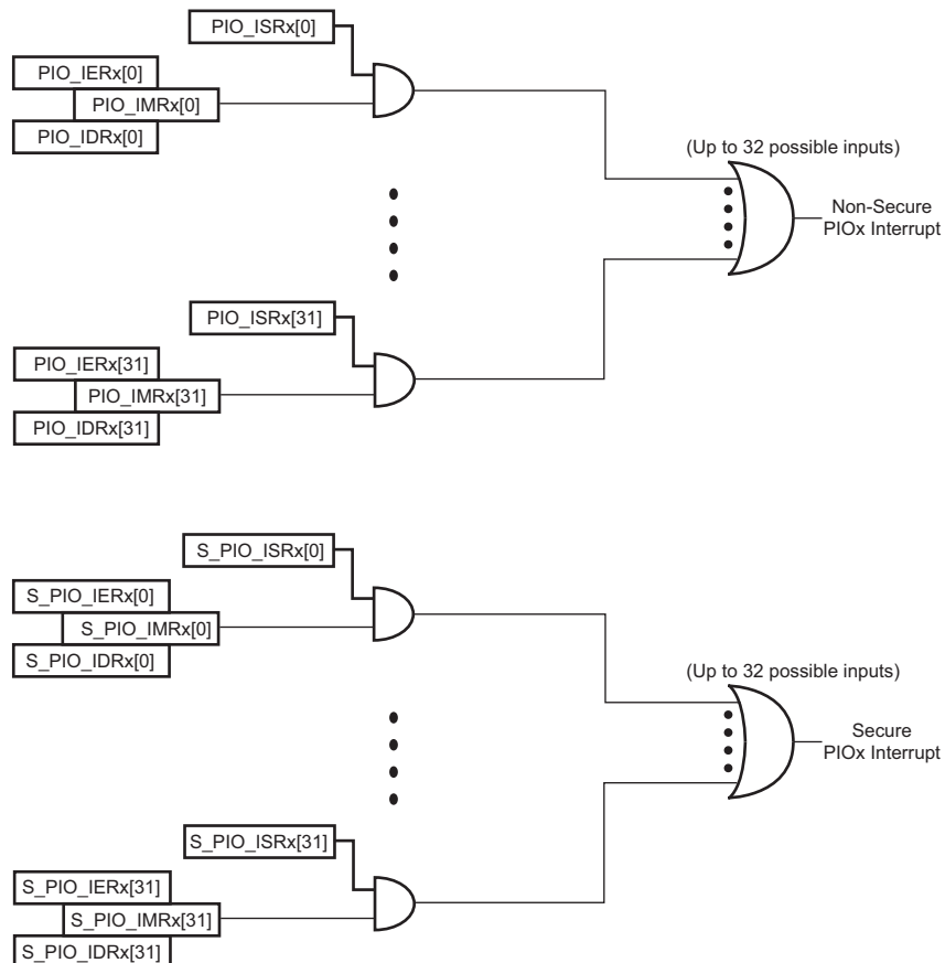
Figure 34-8: PIO Interrupt Management
