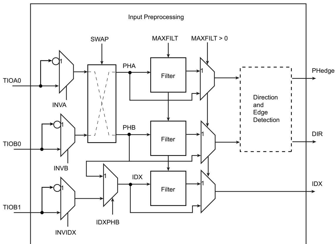
Figure 54-18: Input Stage
