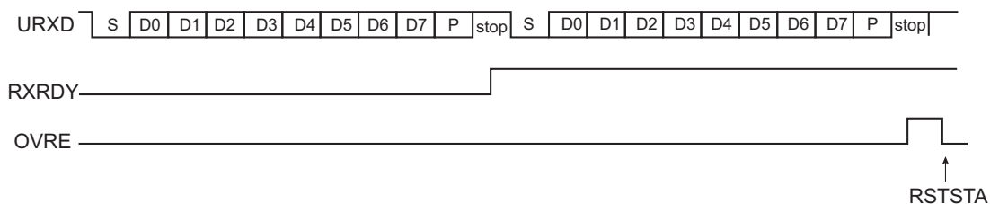
Figure 48-3: Start Bit Detection
