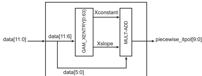
Figure 52-24: Piecewise Linear Interpolation Block Diagram
