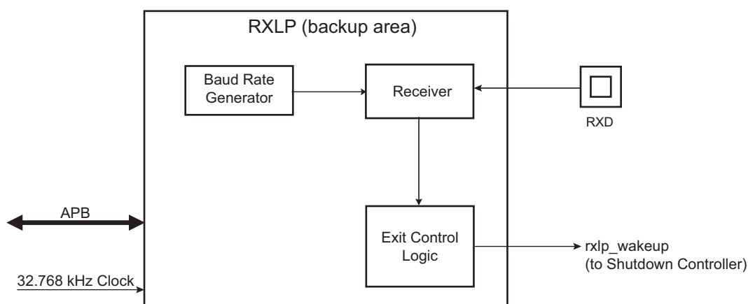
Figure 30-1: RXLP Functional Block Diagram
