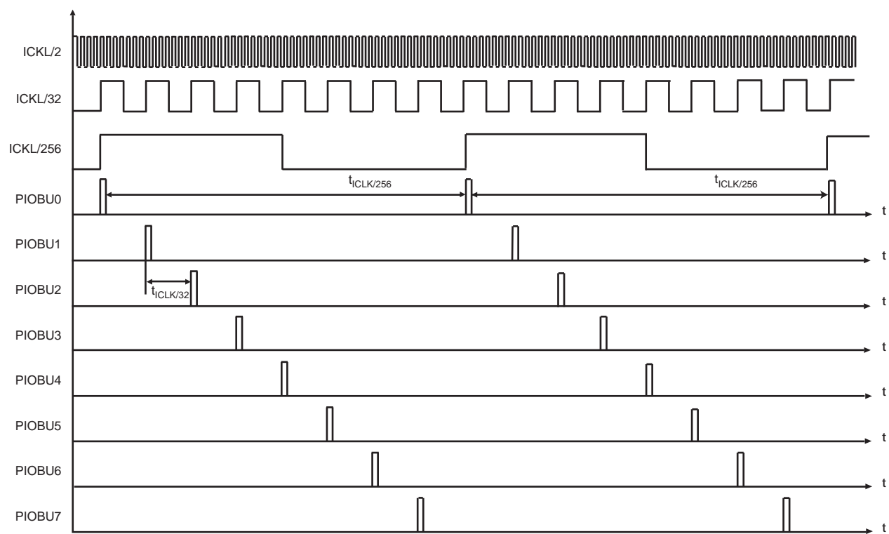
Figure 64-3: Schedule Principle
