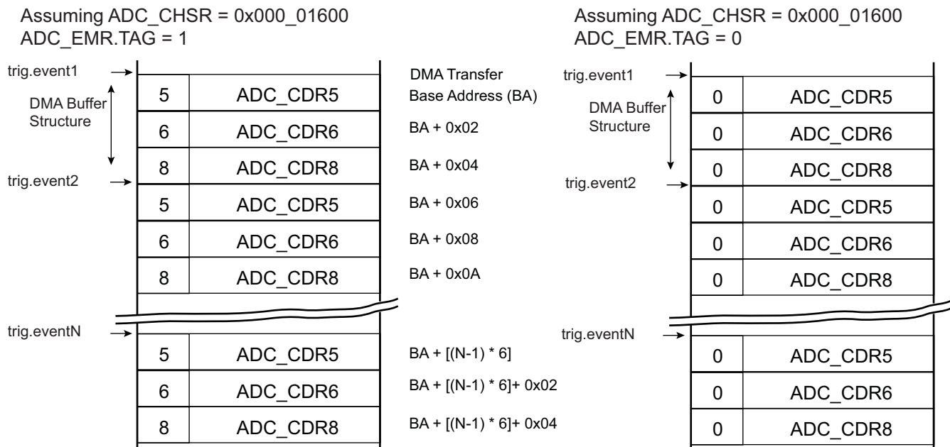
Figure 65-21: Buffer Structure
