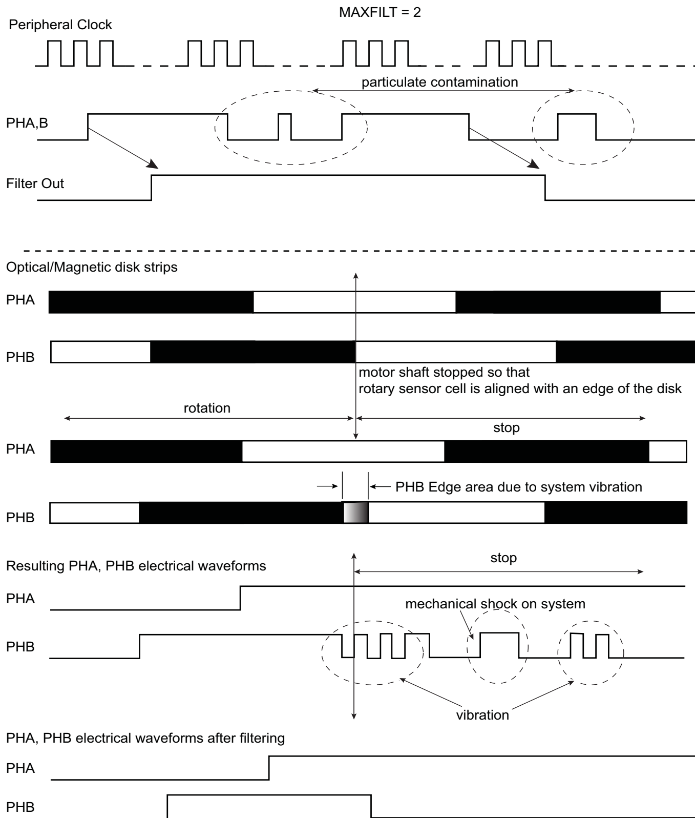
Figure 54-19: Filtering Examples
