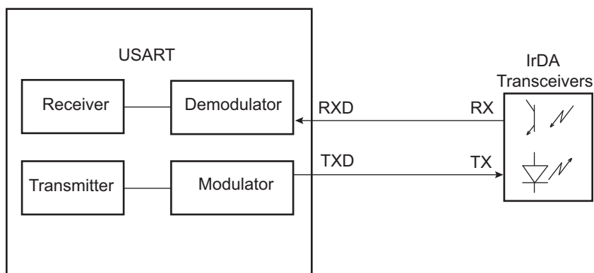
Figure 47-33: Connection to IrDA Transceivers
