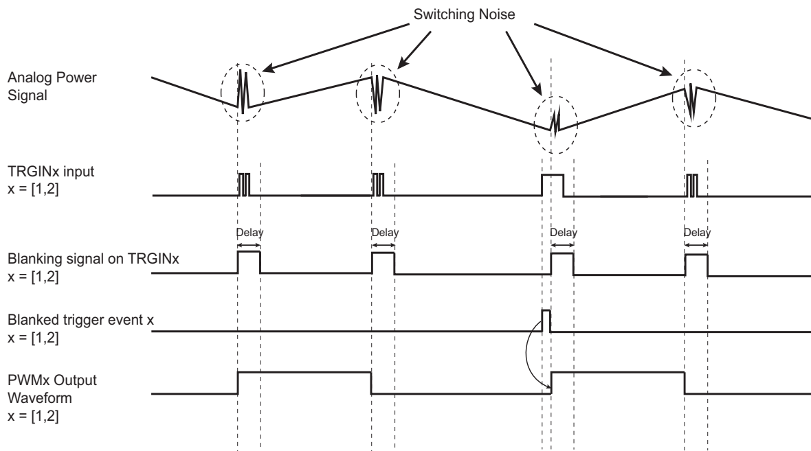
Figure 56-33: Leading-Edge Blanking
