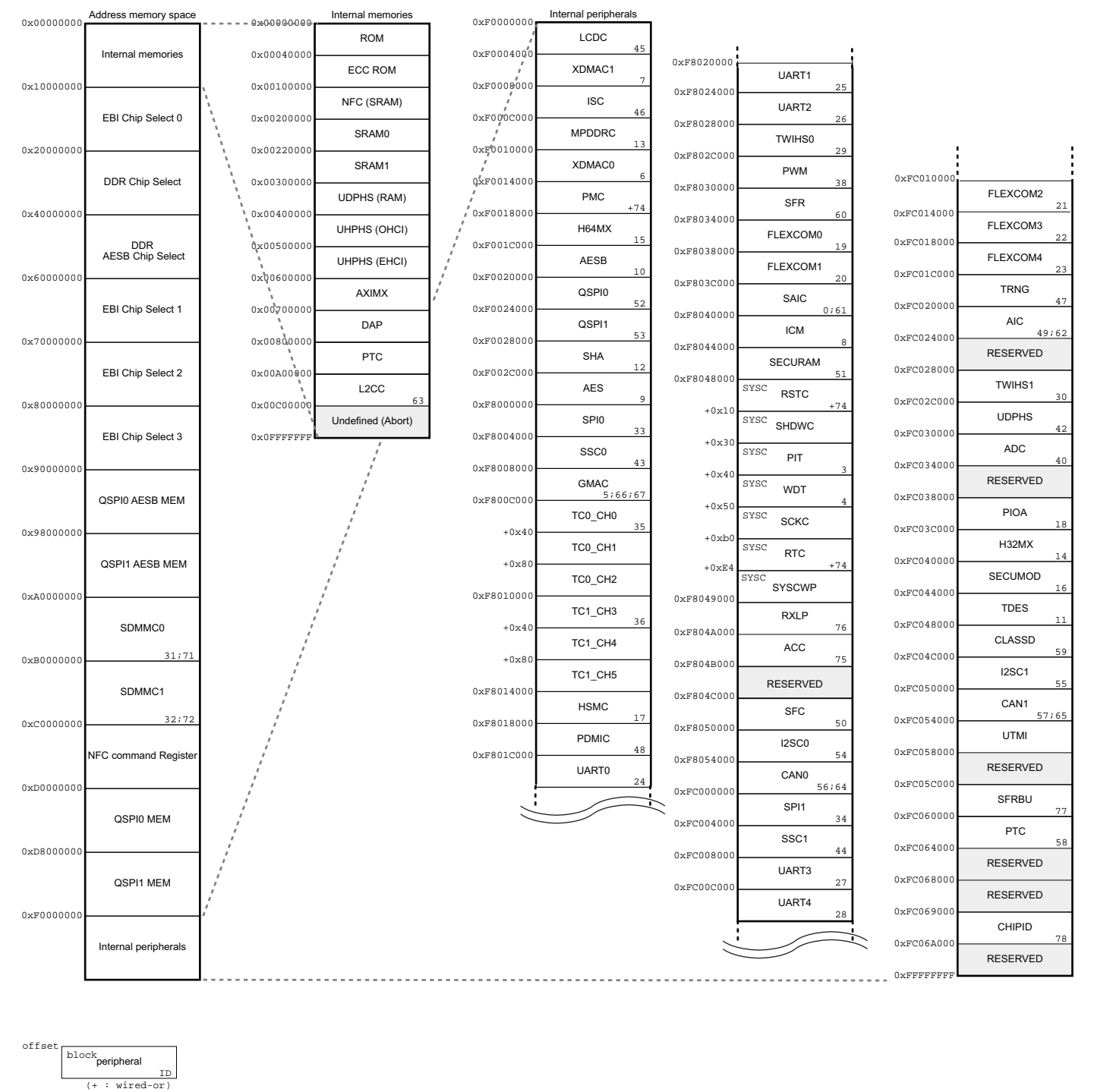
Figure 8-1: Memory Mapping
