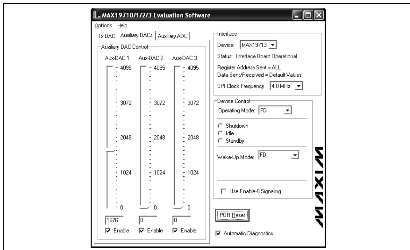
Figure 2. MAX19713 EV Kit Software Auxiliary DAC Control
