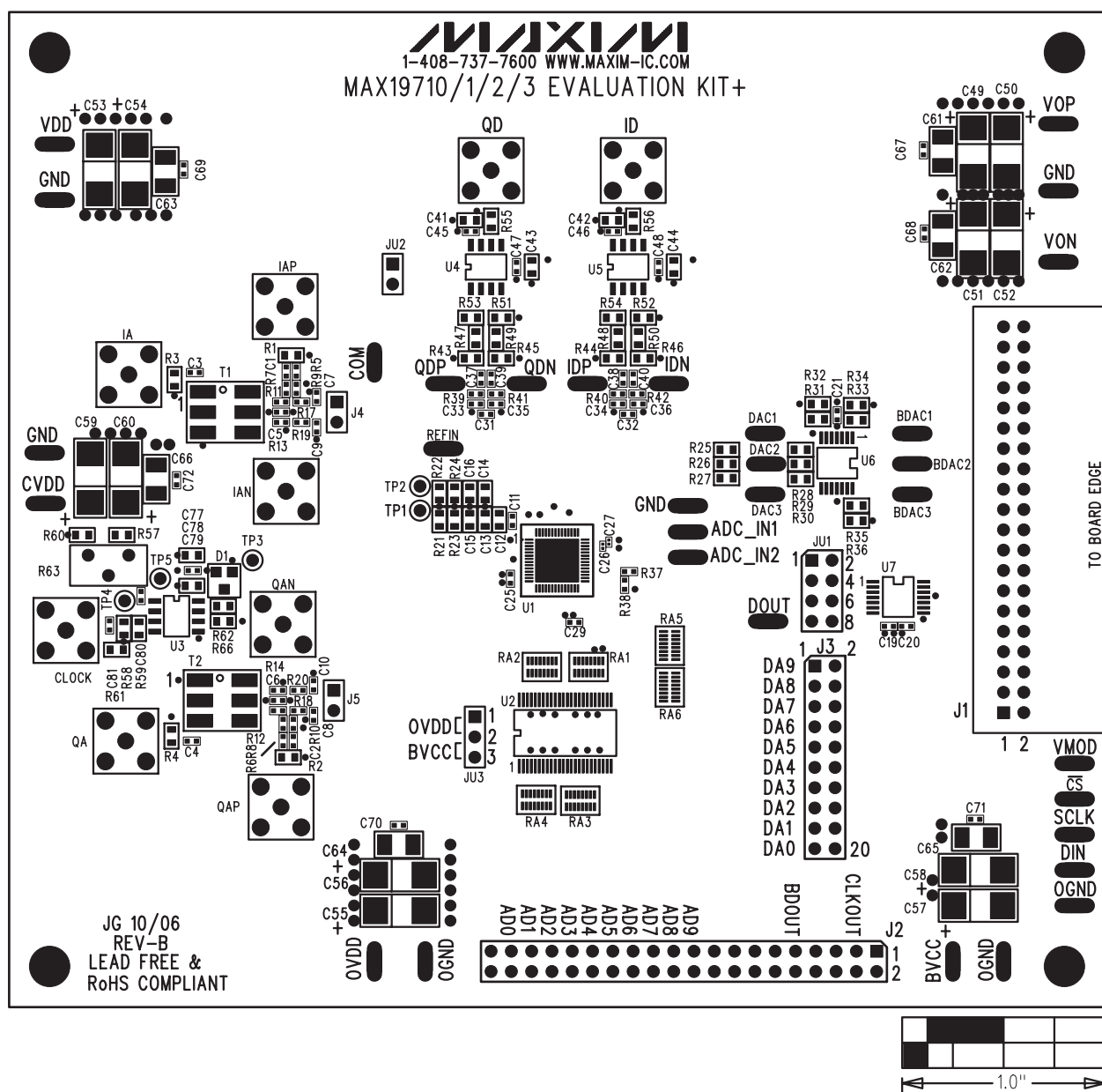
Figure 7. MAX19710–MAX19713 EV Kit Component Placement Guide—Component Side
