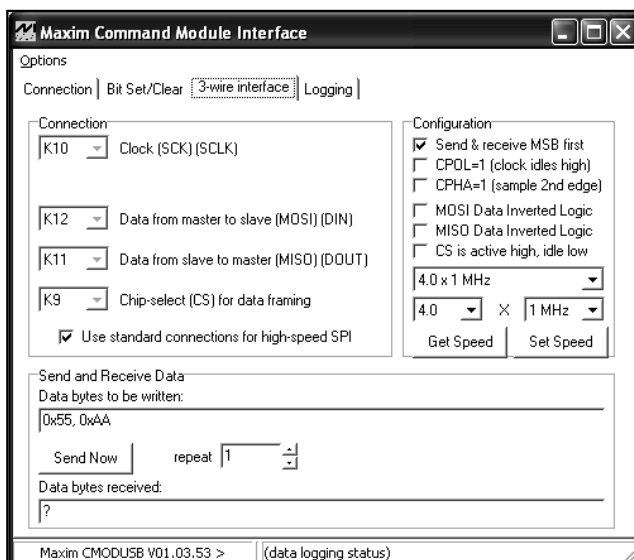
Figure 4. MAX19713 EV Kit Software 3-Wire Interface Diagnostics
