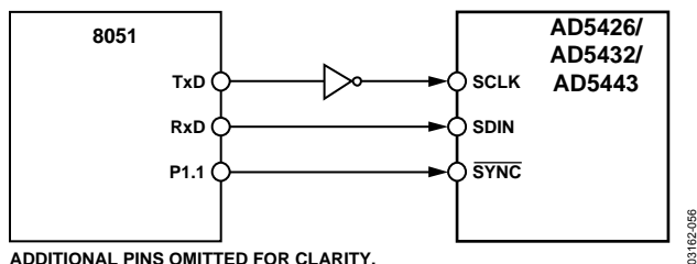
Figure 55. 80C51/80L51-to-AD5426/AD5432/AD5443 Interface
