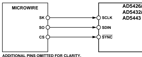
Figure 57. MICROWIRE-to-AD5426/AD5432/AD5443 Interface
