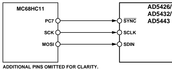
Figure 56. 68HC11/68L11-to-AD5426/AD5432/AD5443 Interface
