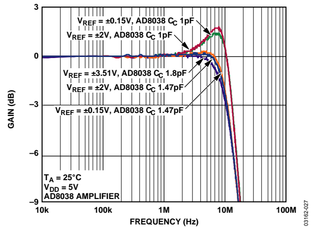
Figure 27. Reference Multiplying Bandwidth vs. Frequency and Compensation Capacitor
