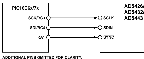
Figure 58. PIC16C6x/7x-to-AD5426/AD5432/AD5443 Interface
