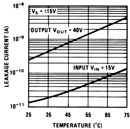
Leakage Currents
