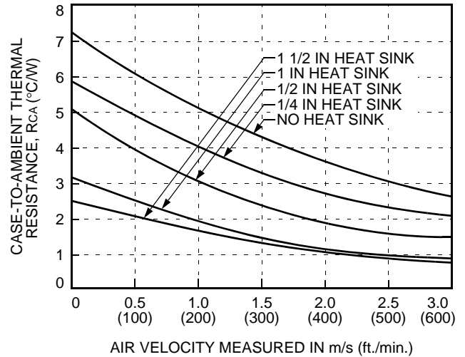
Figure 24. Case-to-Ambient Thermal Resistance Curves; Either Orientation
