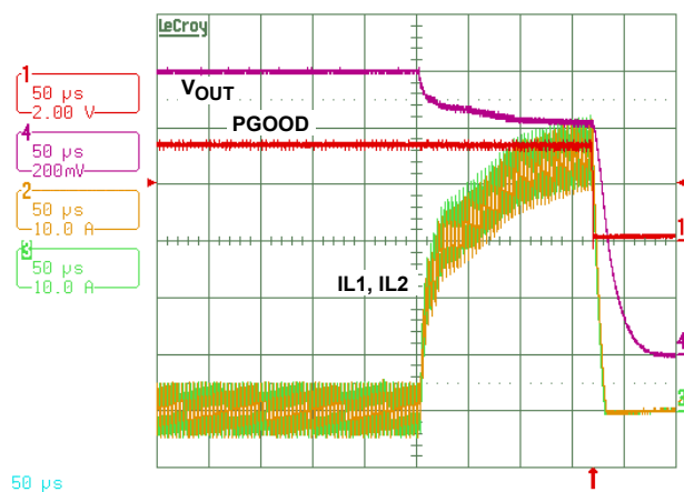
FIGURE 24. OVERCURRENT PROTECTION
