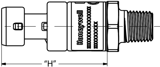
Figure 7. Connector Dimensions (For reference only: mm/[in].)
