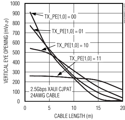
VERTICAL EYE OPENING vs. CABLE LENGTH
