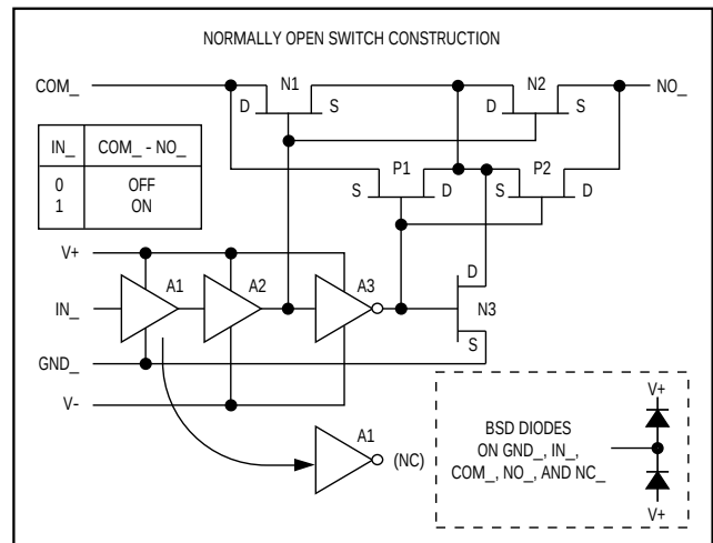
Figure 1. T-Switch Construction
