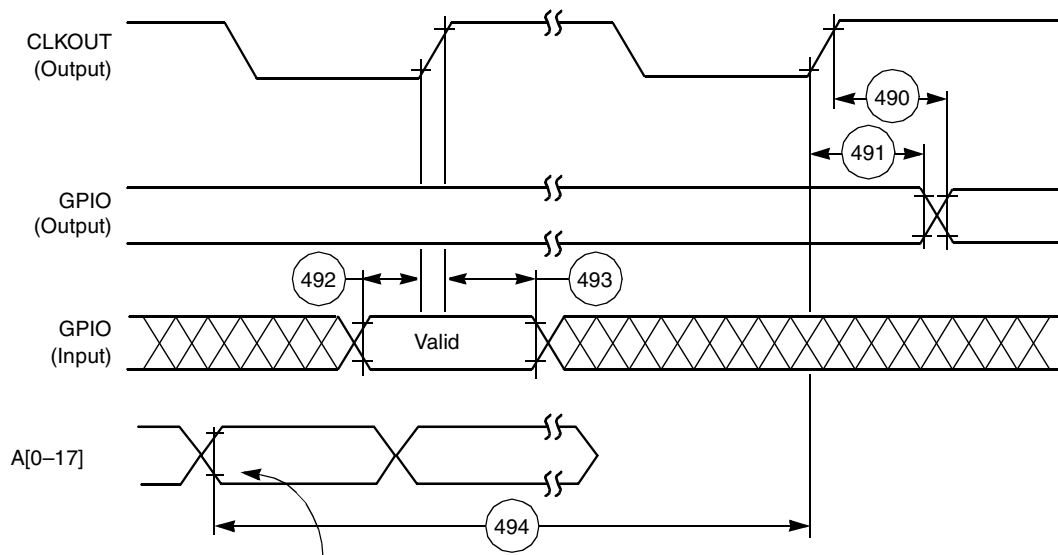
Figure 2-43. GPIO Timing
