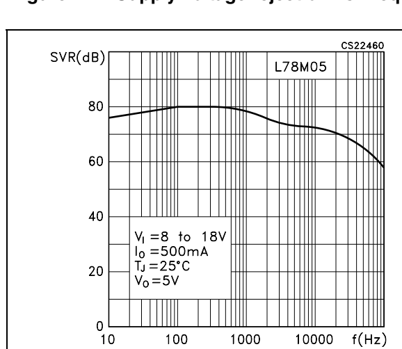
Figure 12. Supply voltage rejection vs. freq.
