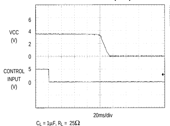
VCC SWITCHING (FALL)
