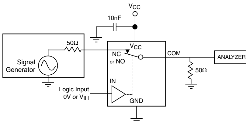
Figure 9. Bandwidth
