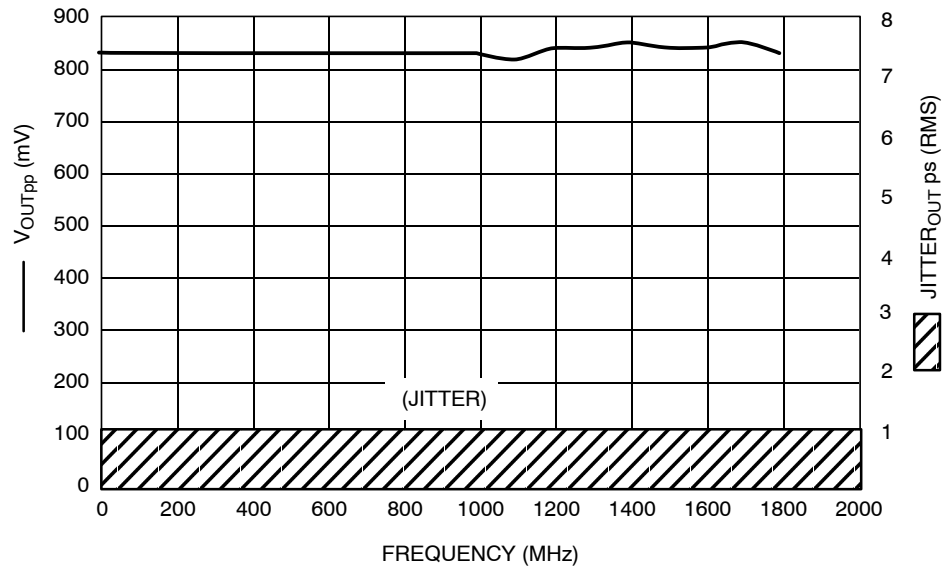
Figure 5. \div 2 , F_{max}/Jitter
