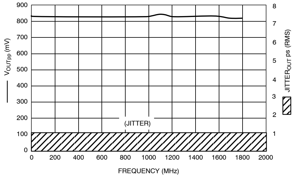
Figure 6. \div 5 , F_{max}/Jitter
