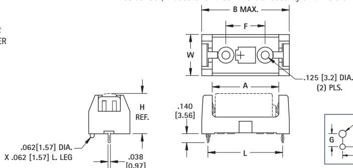
Mounting Detail
