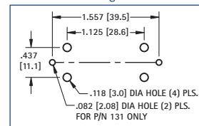
Mounting Detail
