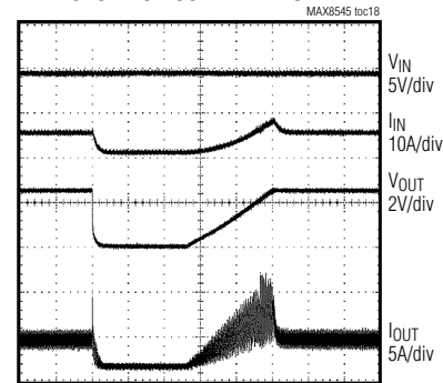
SHORT-CIRCUIT WAVEFORM
