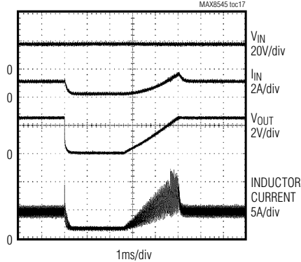
SHORT-CIRCUIT WAVEFORM
