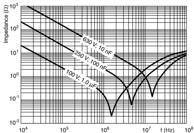
MKT467 - Impedance as a function of frequency (typical curve)
