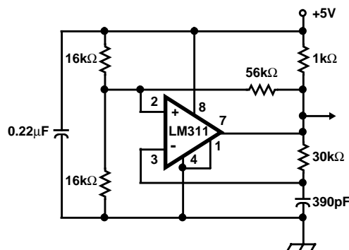
FIGURE 13. LM311 OSCILLATOR
