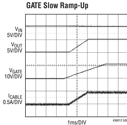
FIGURE 5 CIRCUIT R_{IN} = 150\text{m}\Omega , L_{IN} = 0.7\mu\text{H} \text{LOAD} = 10\Omega , C_{OUT} = 10\mu\text{F}
