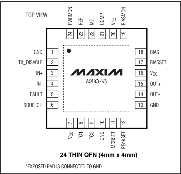
Pin Configuration
