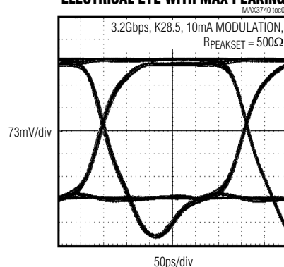
ELECTRICAL EYE WITH MAX PEAKING
