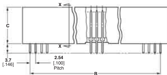
Section Y-Y
