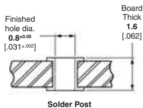
Solder Post
