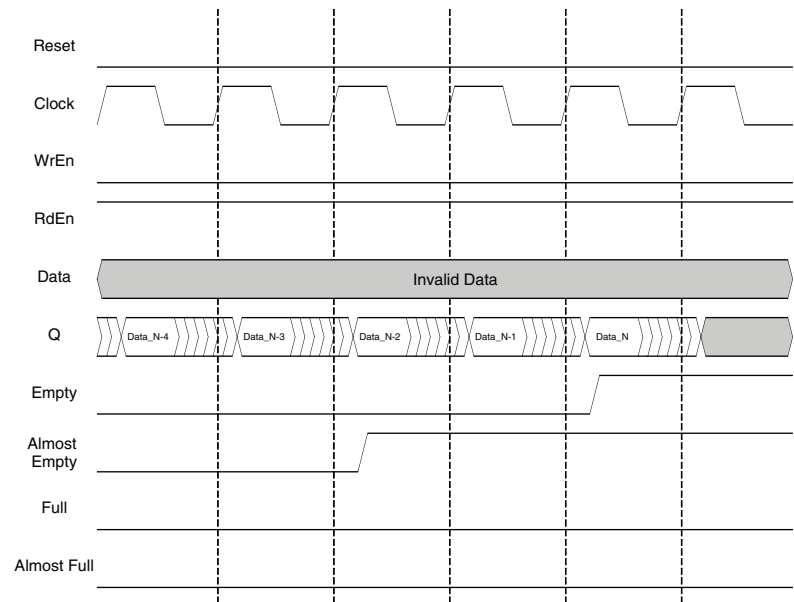
Figure 10-24. FIFO without Output Registers, End of Data Read Cycle
