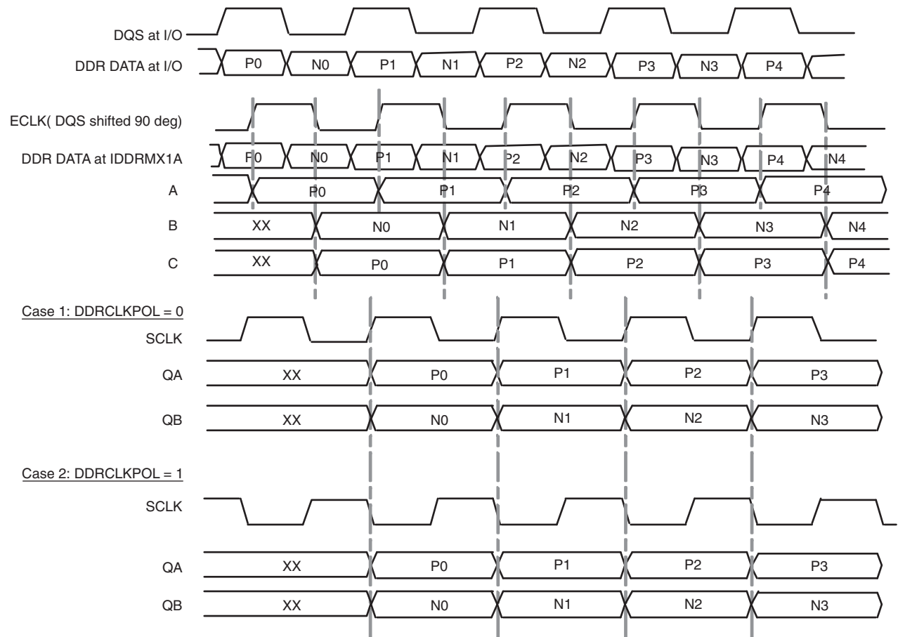
Figure 11-12. IDDRMX1A Waveform
