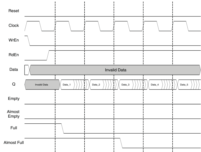
Figure 10-23. FIFO without Output Registers, Start of Data Read Cycle
