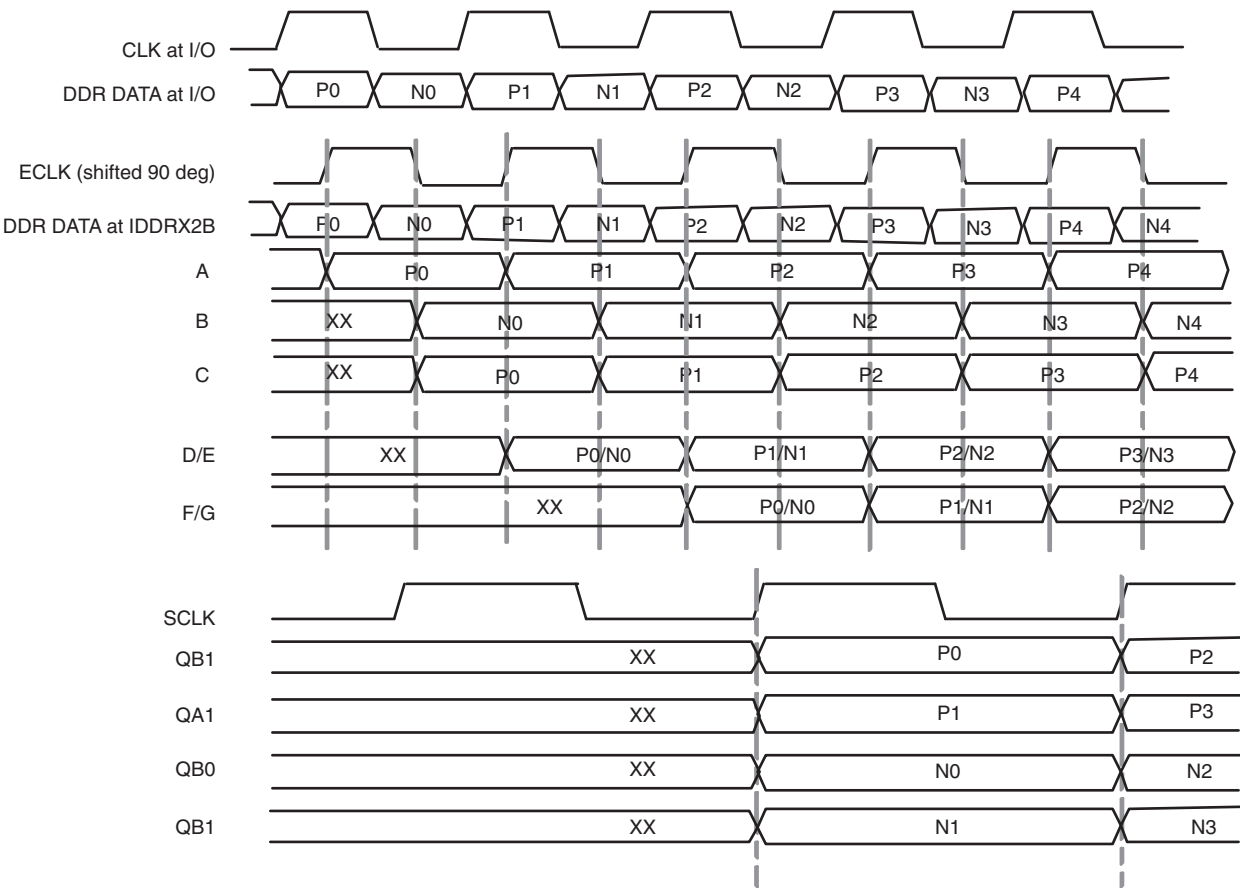
Figure 11-34. IDDRX2B Waveform
