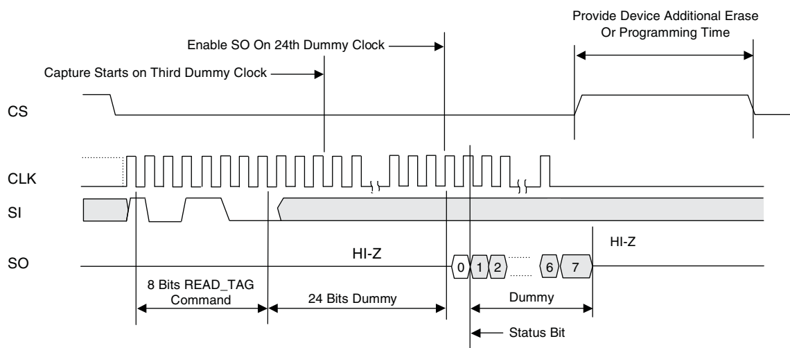
Figure 10-59. STATUS Waveform
