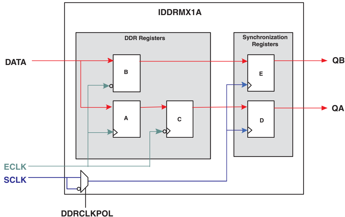
Figure 11-11. Input Register Block in IDDRMX1A Mode
