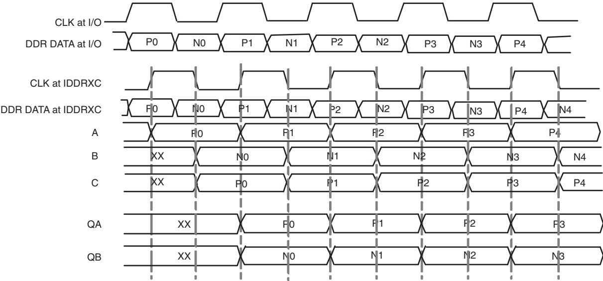
Figure 11-28. IDDRXC Waveform
