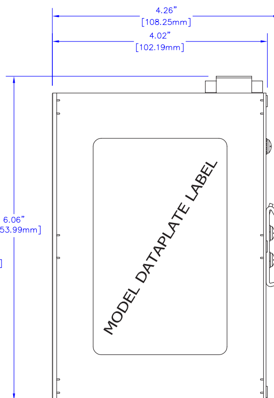
RIGHT SIDE
