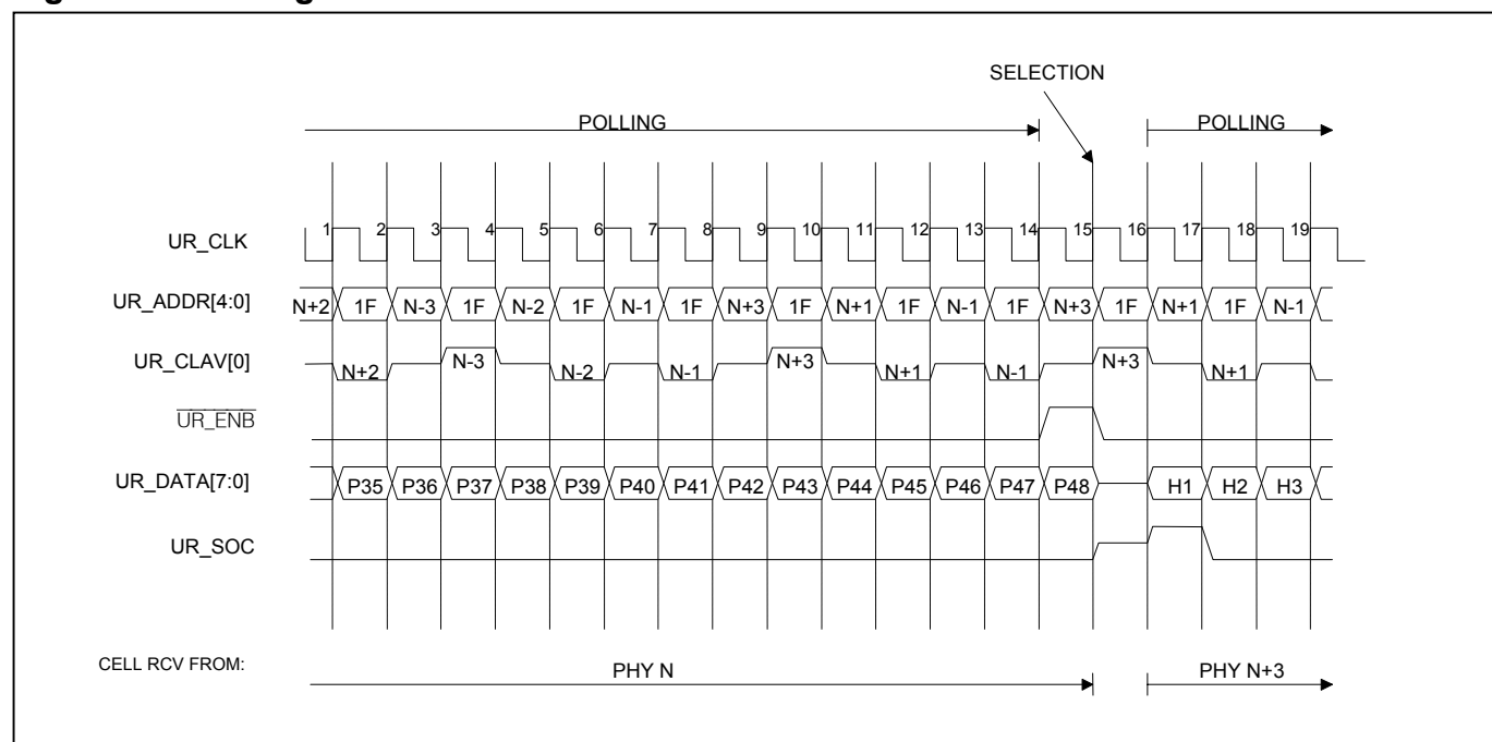
Figure 8-7. Polling Phase and Selection at Receive Interface
