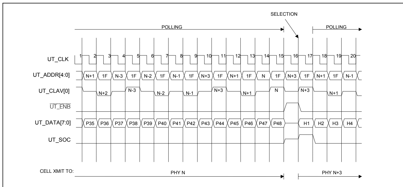
Figure 7-1. Polling Phase and Selection Phase at Transmit Interface
