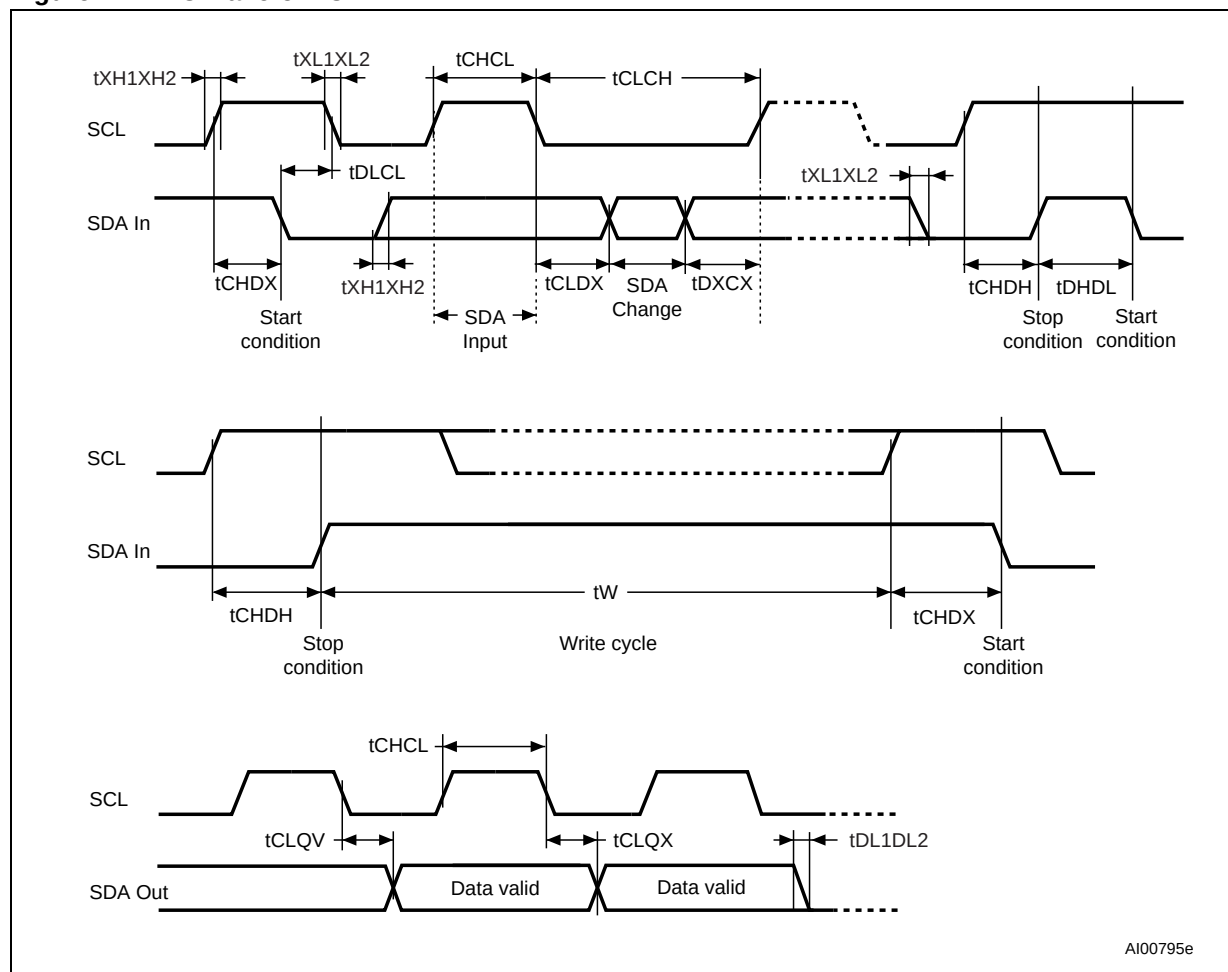
Figure 12. AC waveforms
