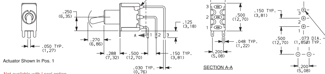
7101MD9AV2BE Horizontal Actuation SPDT
