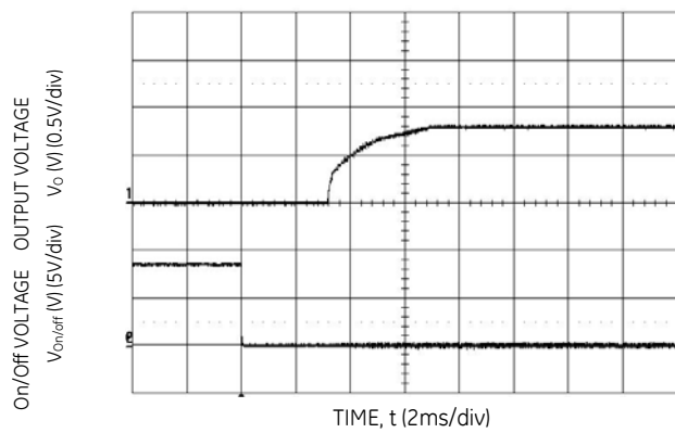
Figure 5. Typical Start-up Using Remote On/Off ( V_{IN} = V_{IN,NOM} , I_o = I_{o,max} ).
