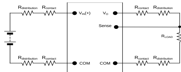
Figure 44. Effective Circuit Configuration for Remote Sense operation.
