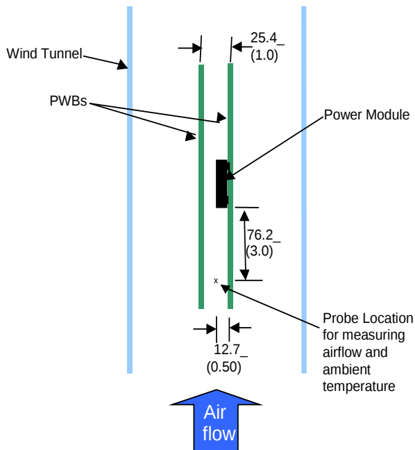
Figure 47. Thermal Test Set-up.
