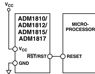
Figure 5. ADM1810/ADM1812/ADM1815/ADM1817 Typical Application
