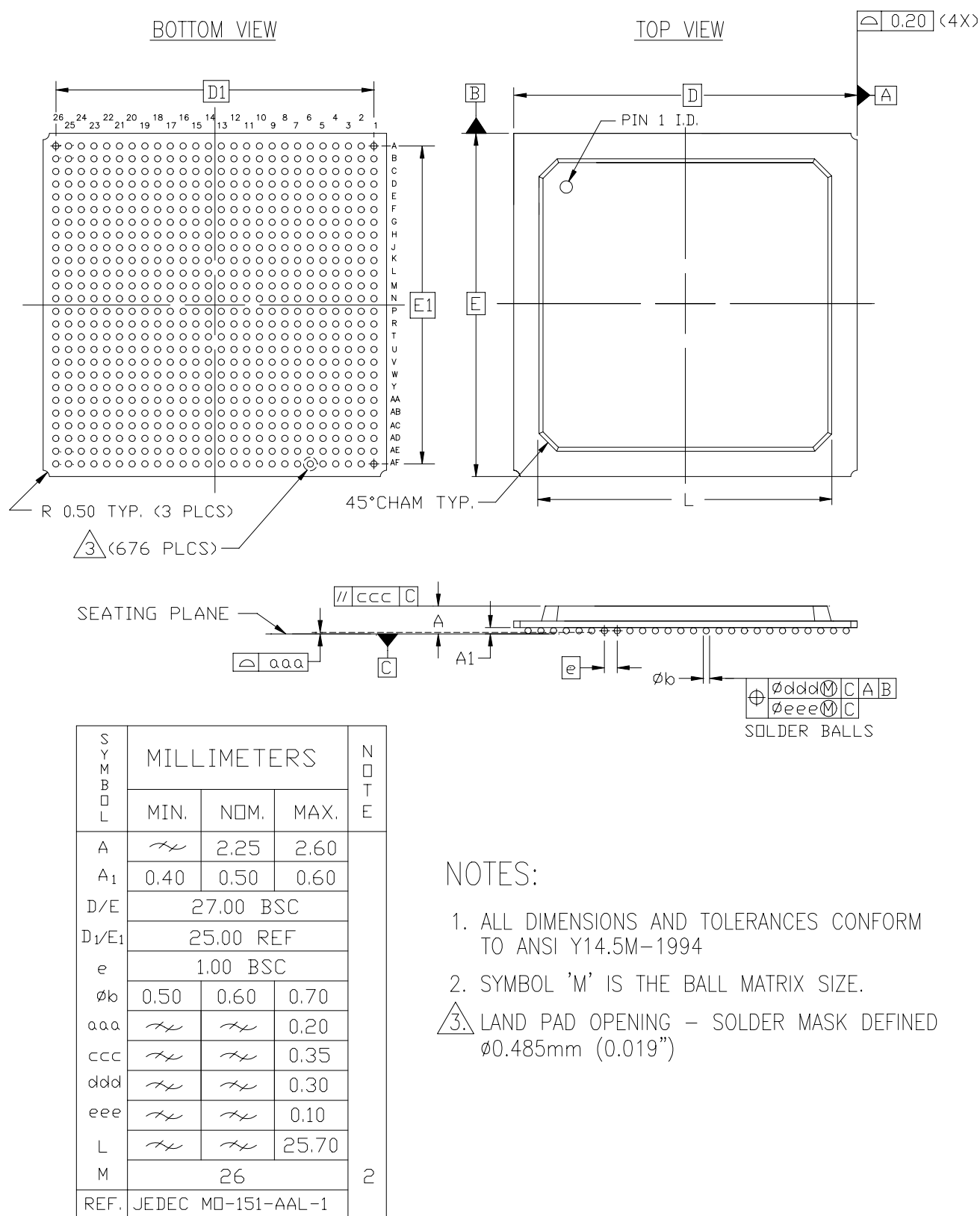
Figure 4: FG676 Fine-Pitch BGA Package Specifications
