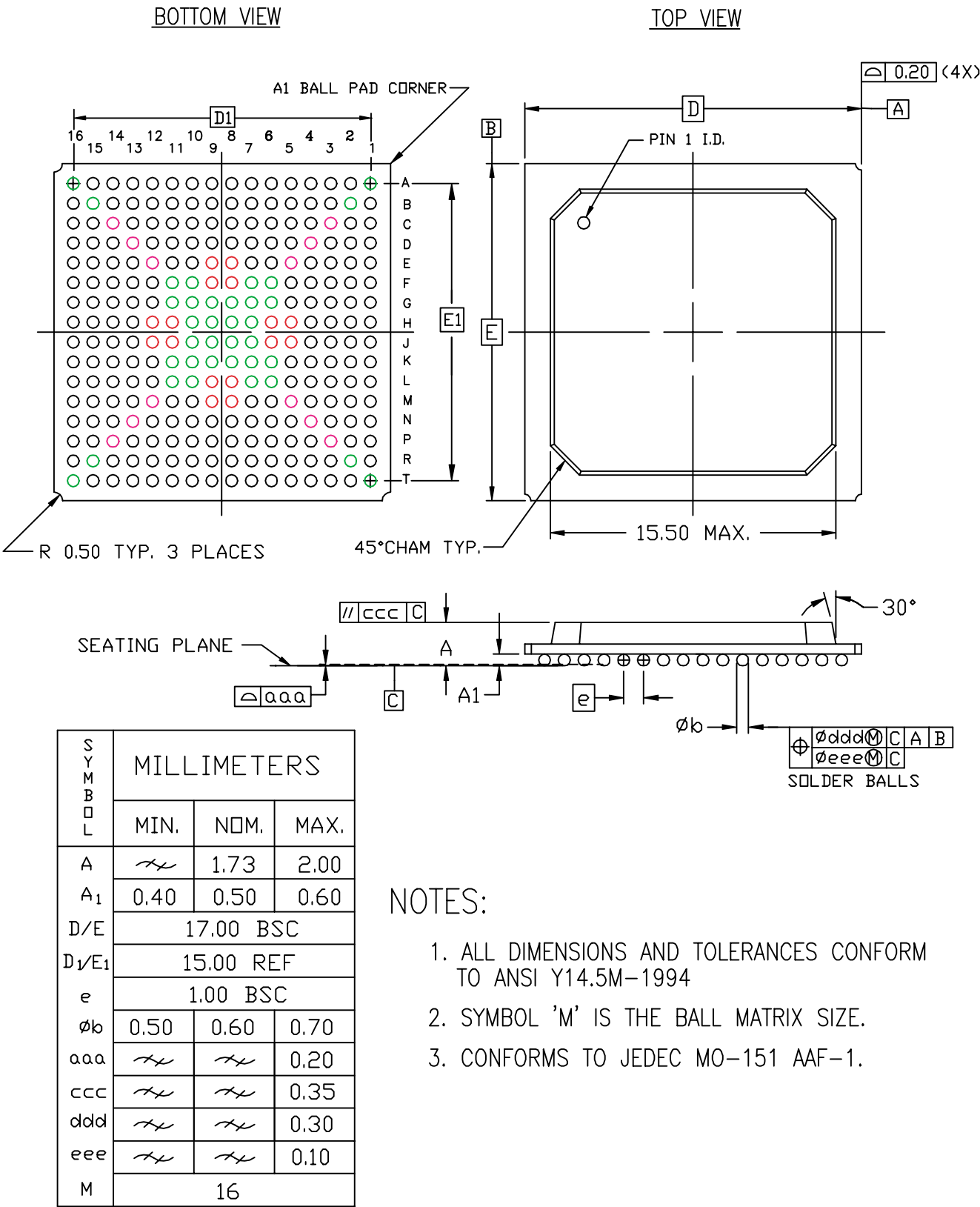
Figure 2: FG256 Fine-Pitch BGA Package Specifications
