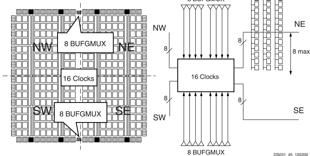
Figure 39: Virtex-II Clock Distribution
