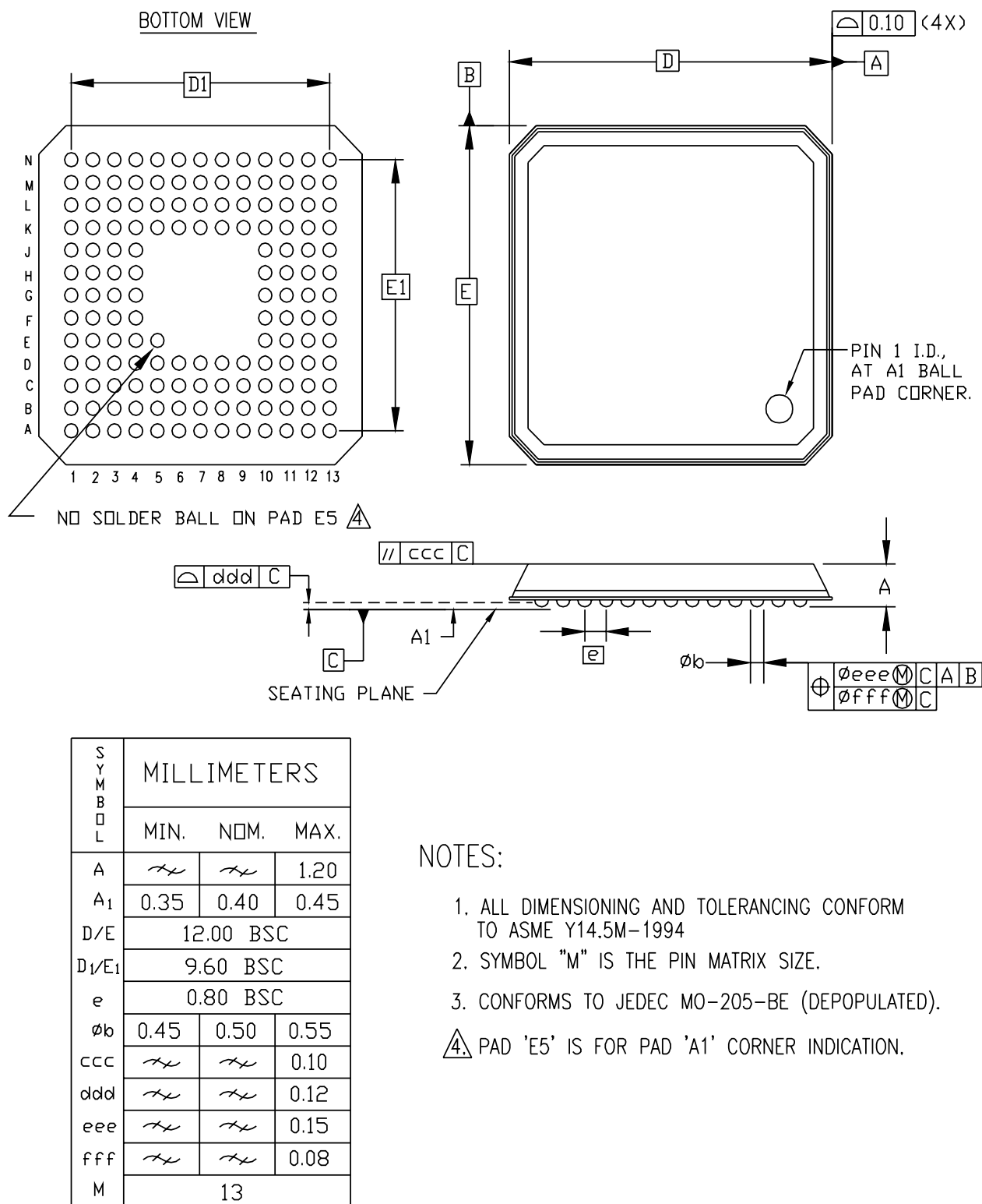
Figure 1: CS144 Chip-Scale BGA Package Specifications
