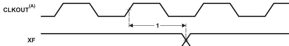
Figure 5-20. XF Timings
