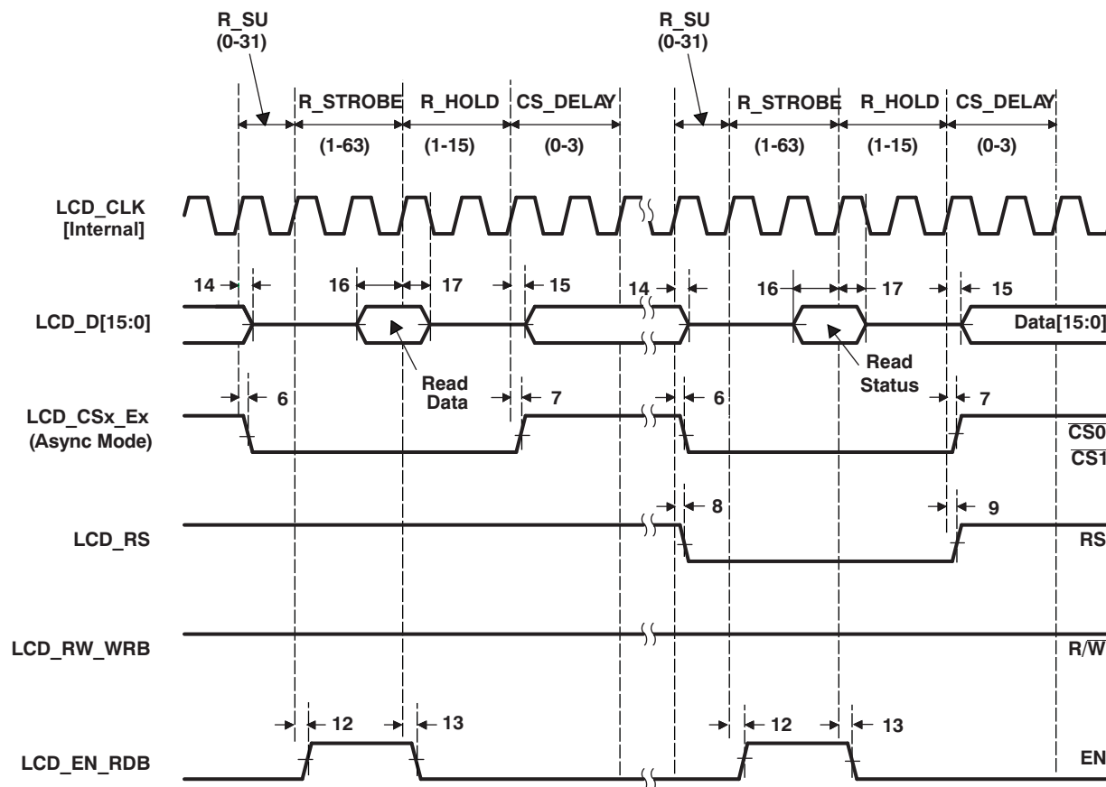
Figure 5-29. Micro-Interface Graphic Display 6800 Status
